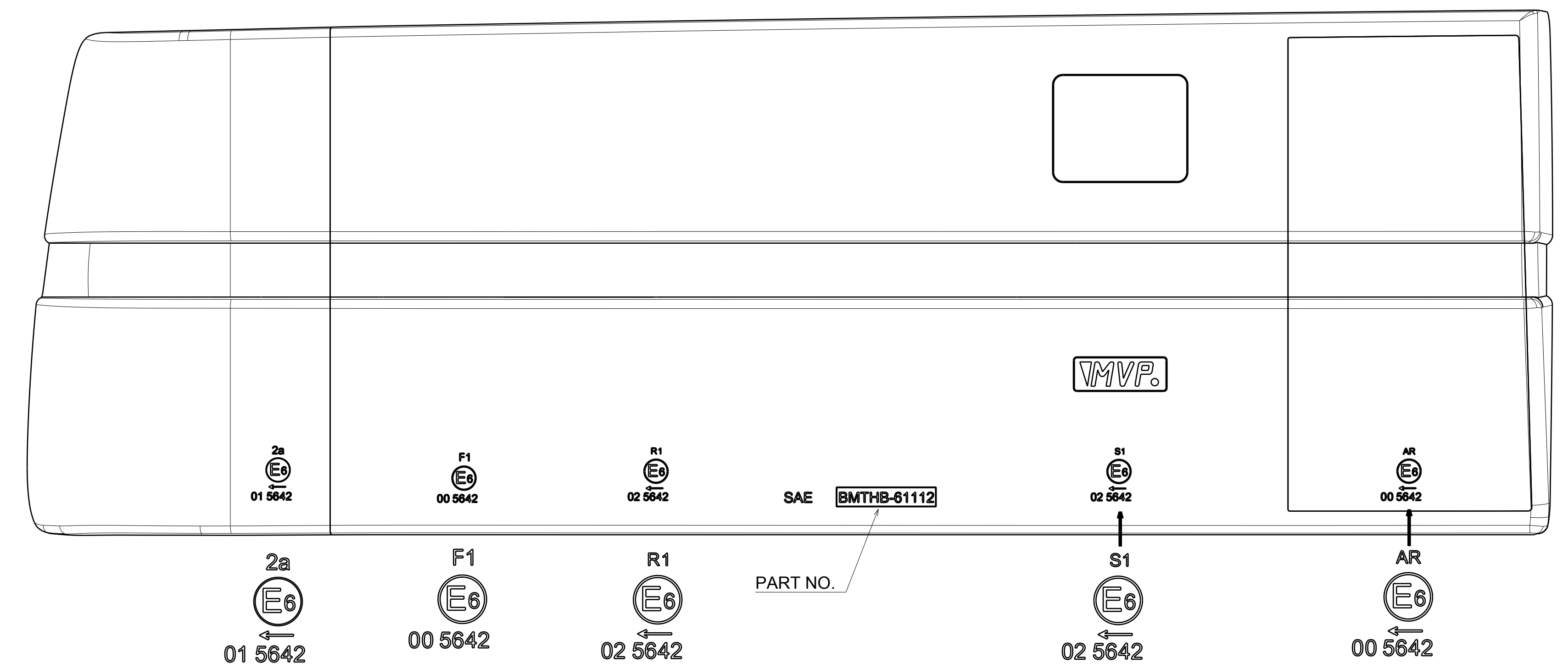
LENS-ENGRAVING-(E-MARK)-LH
