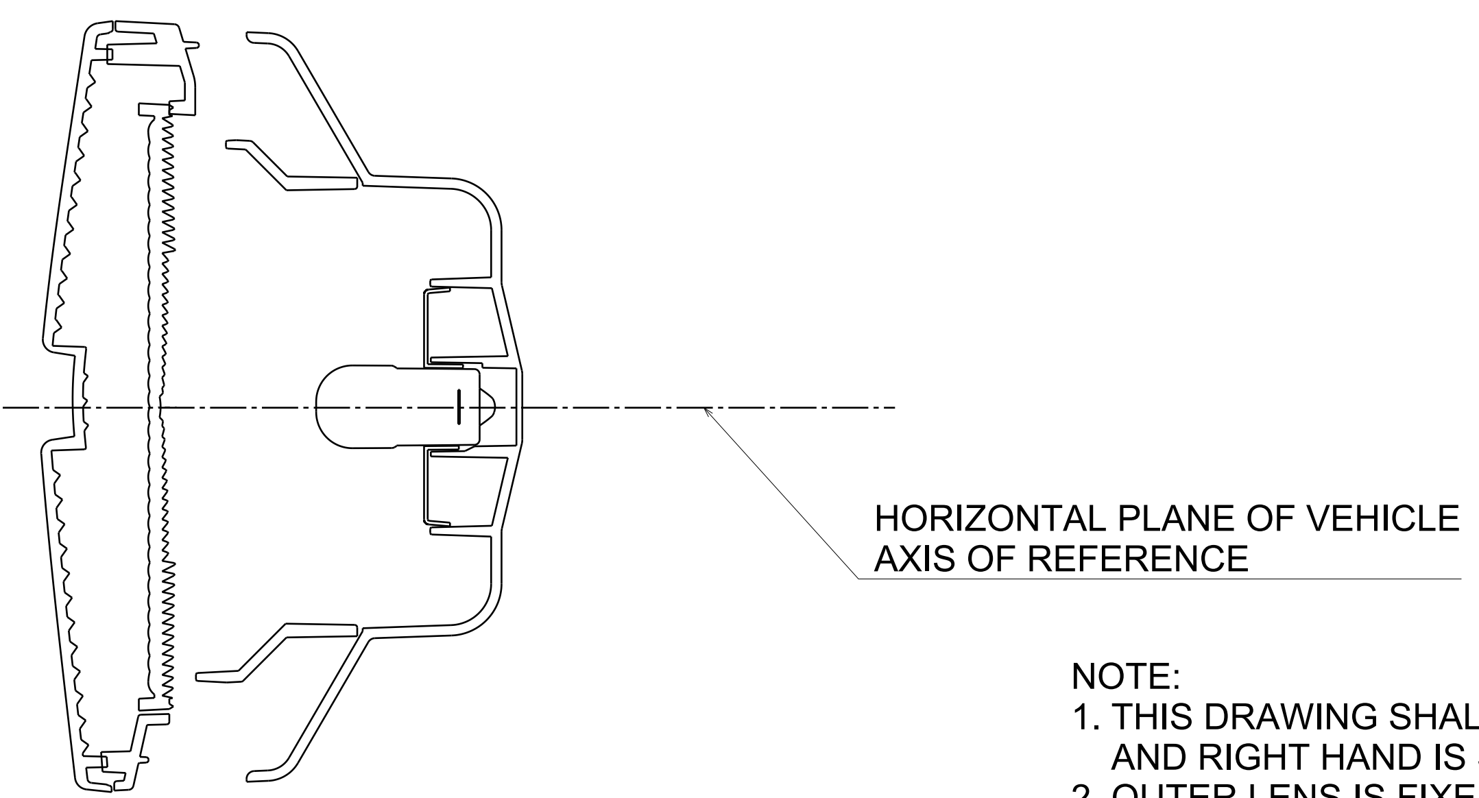
SECTION B-B
