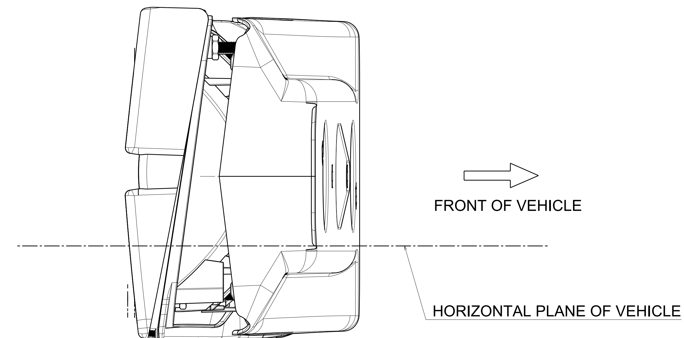
SIDE VIEW
